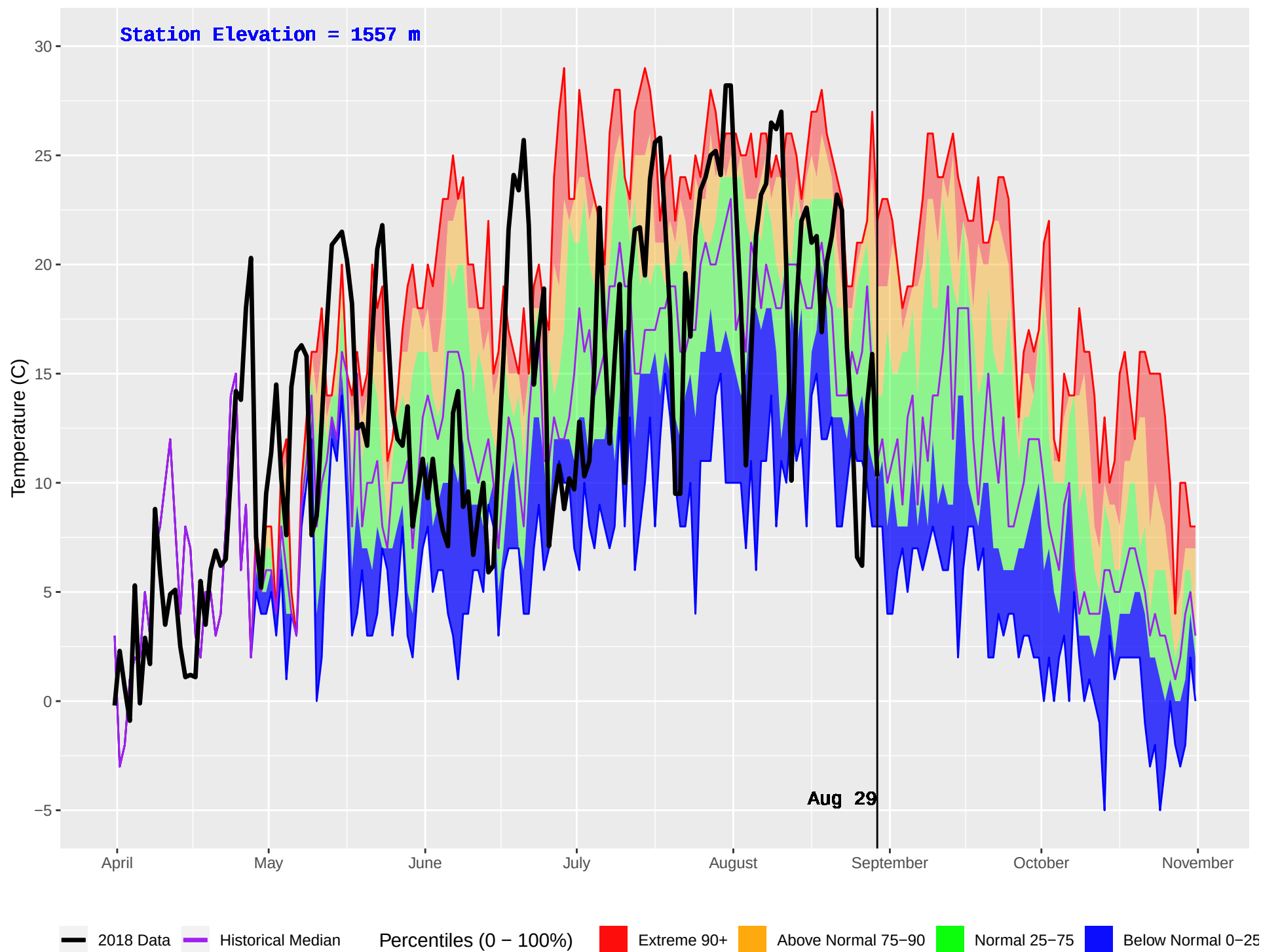
SKOONKA (1024) : Historical (2008–2016) and Current (2018) Daily Temperature
